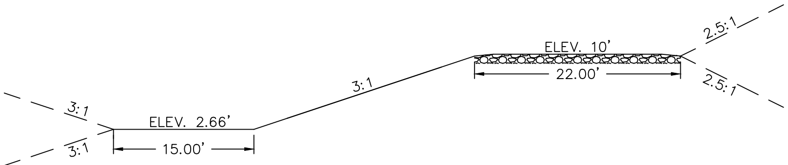
TYPICAL CROSS SECTION (STA 8+00) SCALE: 1"=10'
