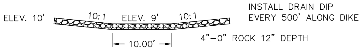
TYPICAL DRAIN DIP SCALE: 1"=10'
