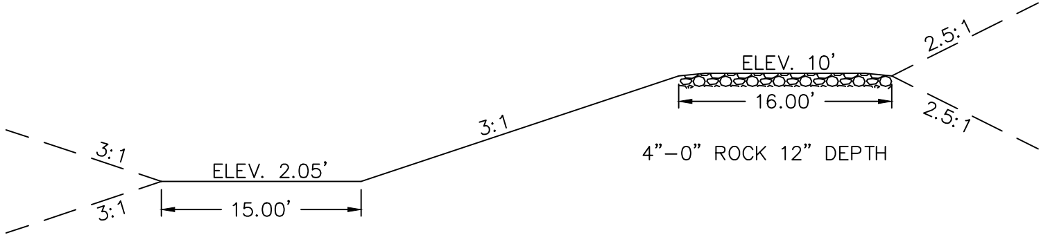
TYPICAL CROSS SECTION (STA 15+39) SCALE: 1"=10'
