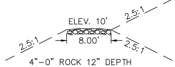
TYPICAL CROSS SECTION (ACCESS DIKE) SCALE: 1"=10'
