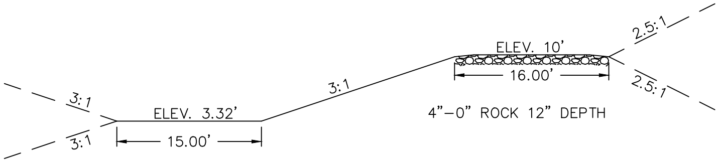
TYPICAL CROSS SECTION (STA 0+00) SCALE: 1"=10'
